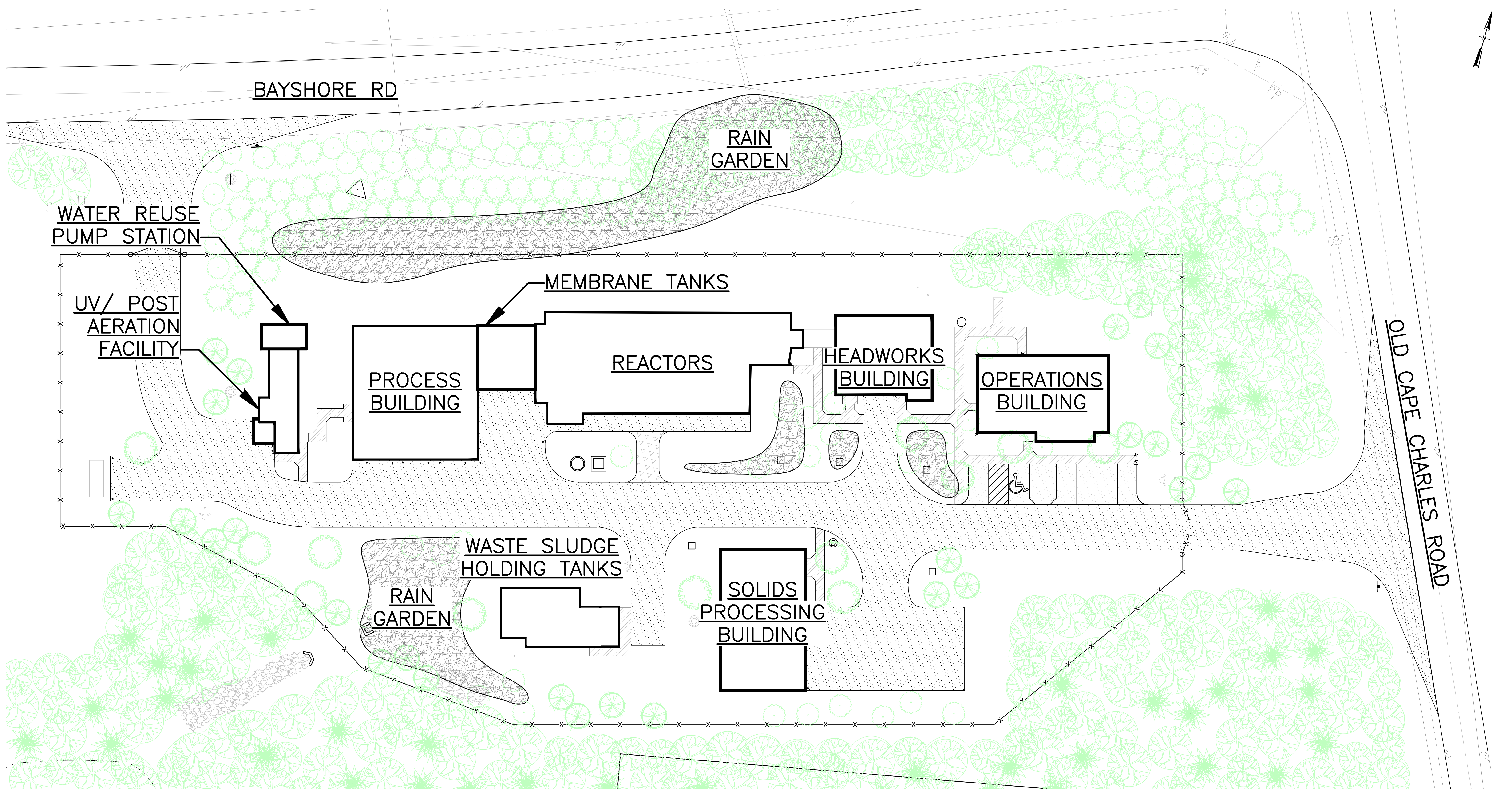
WASTEWATER TREATMENT PLANT SITE PLAN
